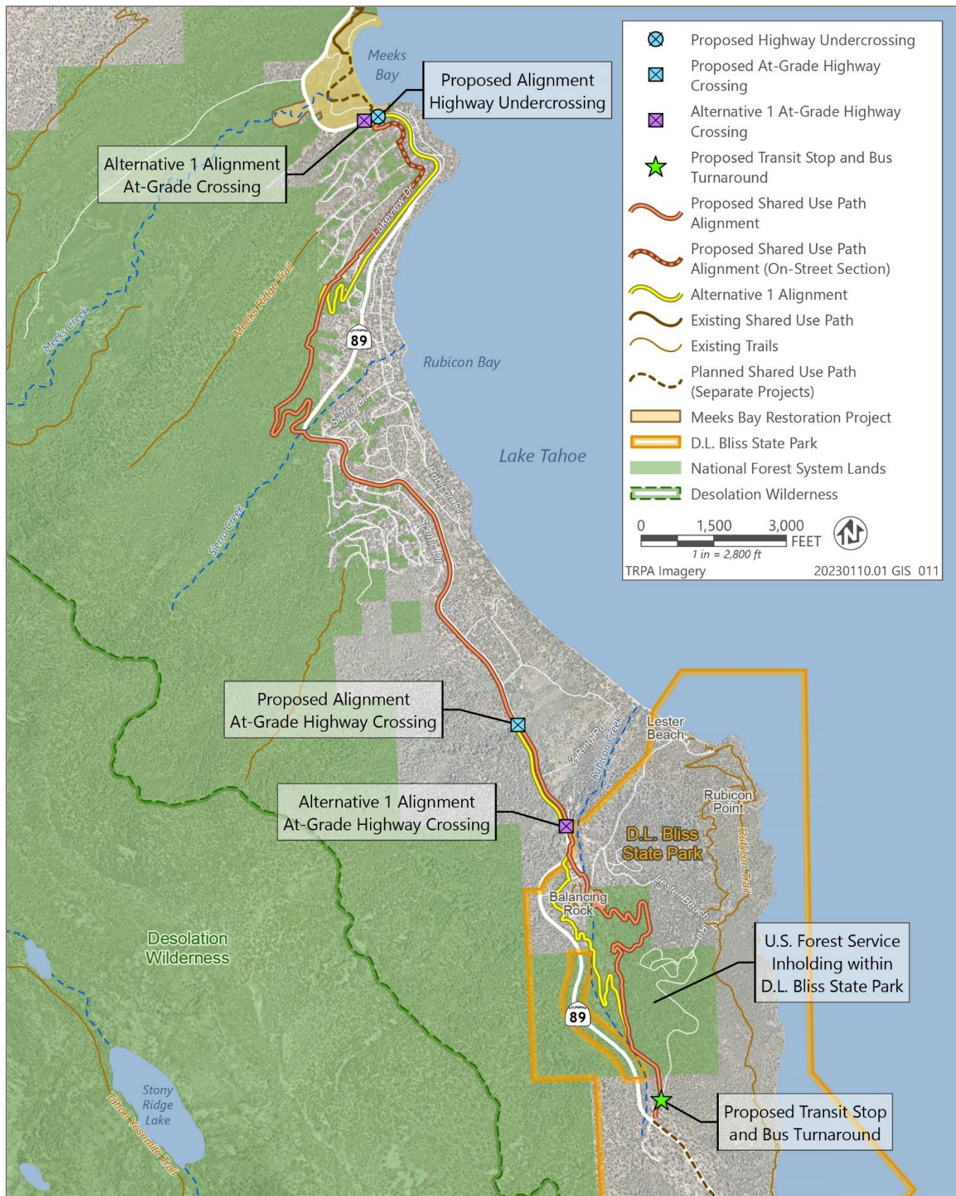
Figure 2 West Shore Trail – Meeks Bay to D.L. Bliss Shared Use Path Alignments
