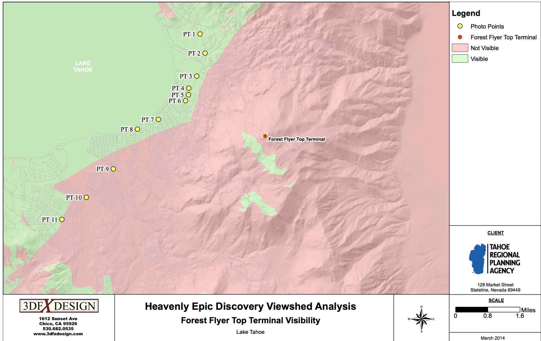
Figure 3.10-4 Viewshed Analysis – Forest Flyer Top Terminal Visibility
